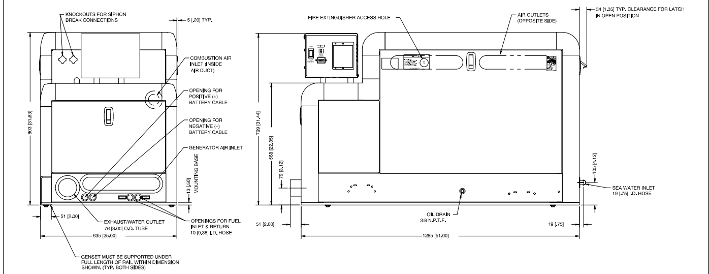
ADV-6285B-E
